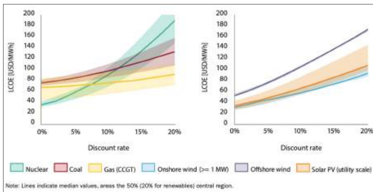
Fig. 2 - LCOE as a function of the discount rate
